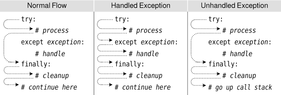
图 4-2 Try ... except ... finally 控制流
